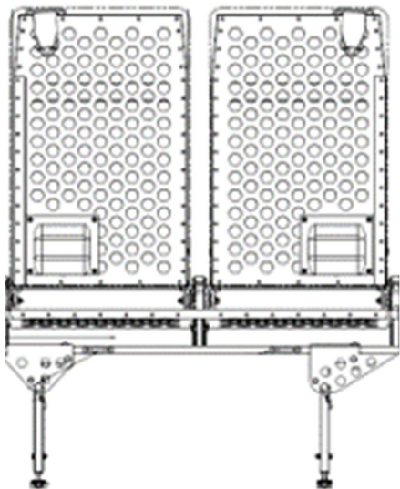
Forward View
